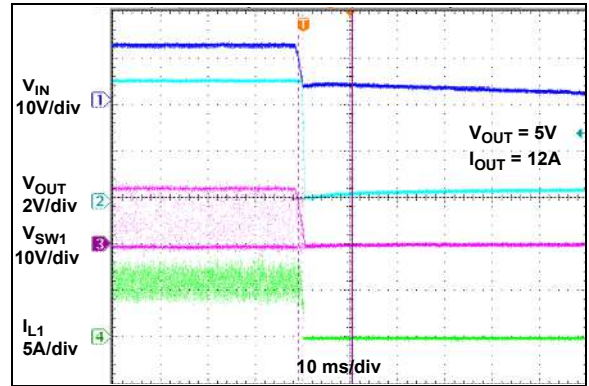
FIGURE 2-46: Power-Down with V_{IN} and 12A Load.
