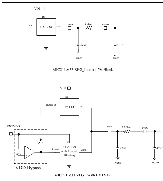
FIGURE 4-14: MIC21LV33 EXTVDD.
