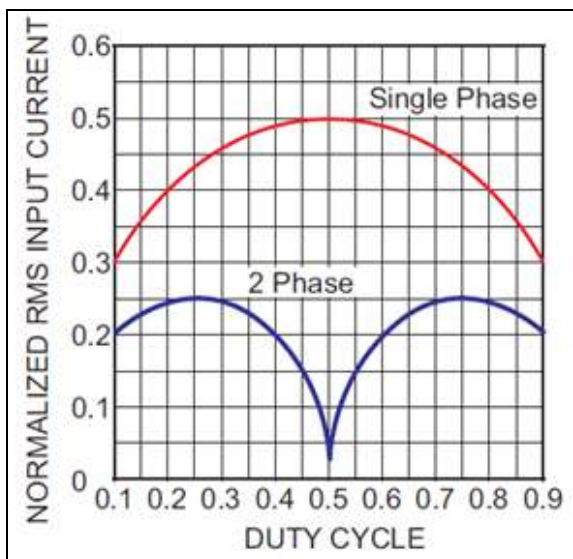
FIGURE 5-2: Normalized RMS Input Capacitor Current vs. Duty Cycle.
