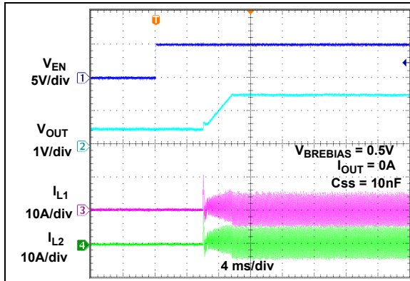
FIGURE 2-31: Pre-Bias Start-up ( V_{IN} = 12V , V_{OUT} = 1.5V , V_{PREBIAS} = 0.5V ).
