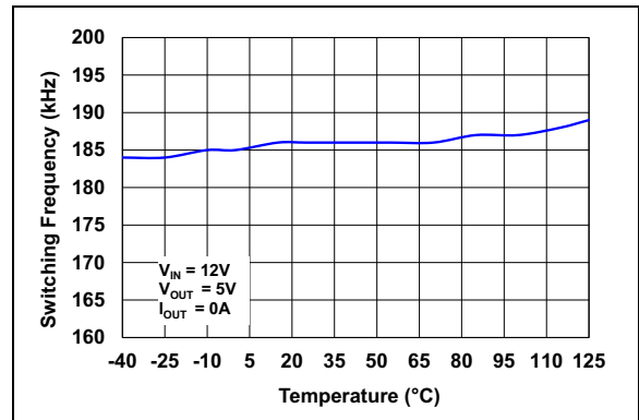
FIGURE 2-11: Switching Frequency per Phase vs. Temperature.
