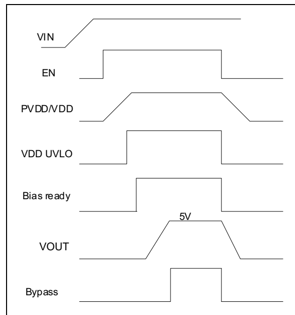
FIGURE 4-15: EN Pin Sequencing.
