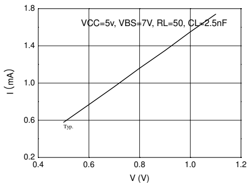
Figure 14. Recharge FET I-V curve
