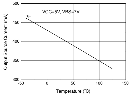
Figure 5b. Output Source Current vs Temperature
