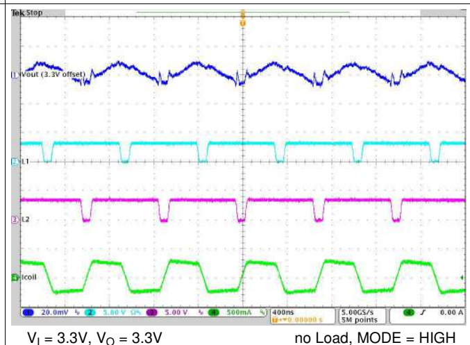
Figure 19. Switching Waveforms, PWM Buck-Boost Operation
