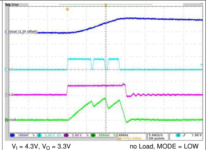
Figure 23. Switching Waveforms, PFM Buck Operation
