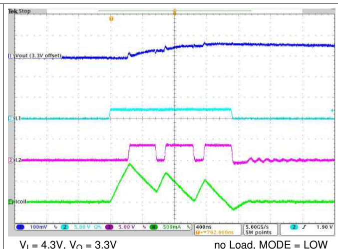
Figure 21. Switching Waveforms, PFM Boost Operation
