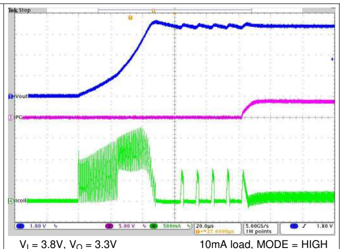
Figure 27. Softstart Waveforms in forced PWM Mode
