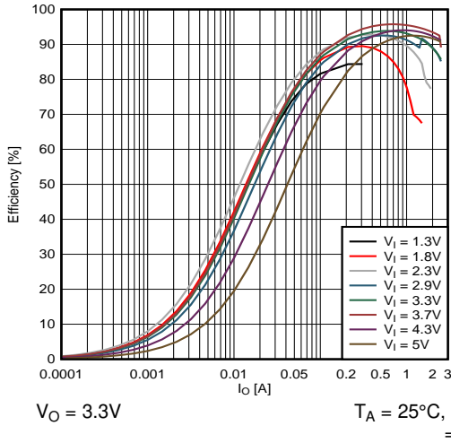
Figure 16. Efficiency vs. Output Current
