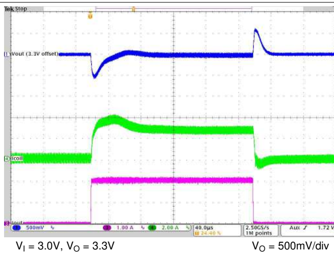
Figure 35. 2A-Loadstep Waveforms
