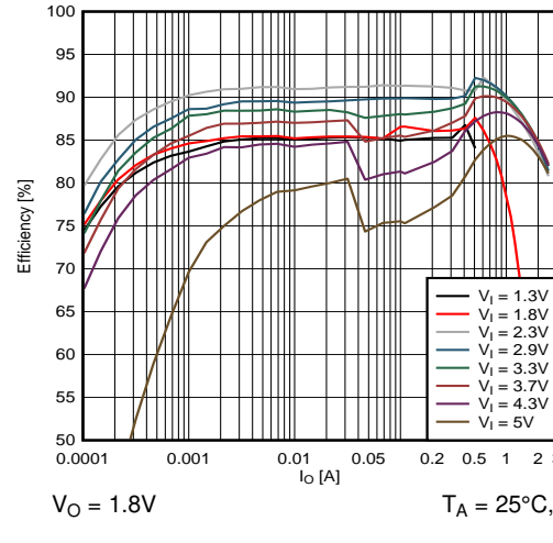
Figure 17. Efficiency vs. Output Current
