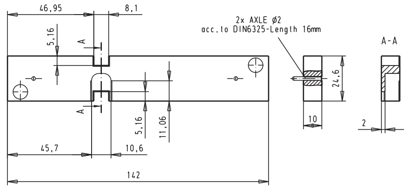
Part 3: har.mik RIGHT GUIDE
