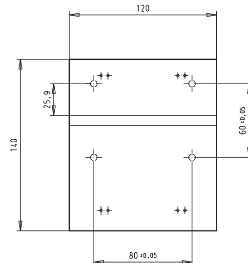
Part 1: har-mik BASE PLATE
