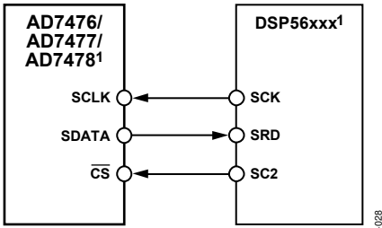
Figure 28. Interfacing to the DSP56xxx
