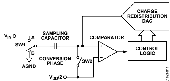
Figure 11. ADC Conversion Phase
