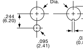
MTA8106DVRA Vertical Actuation
