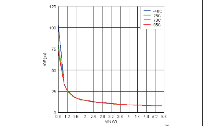
Figure 17. V_{IN} vs t_{OFF} ( V_{BIAS} = 5.5\text{ V} , C_T = 1\text{ nF} )
