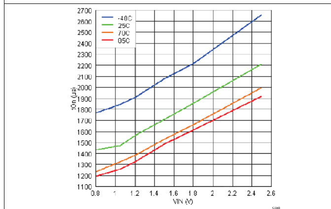
Figure 18. V_{IN} vs t_{ON} ( V_{BIAS} = 2.5\text{ V} , C_T = 1\text{ nF} )
