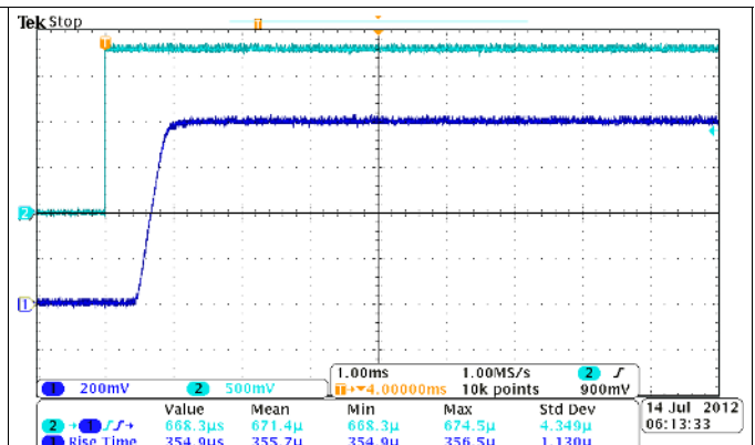
Figure 24. Turnon Response Time (V_{IN} = 0.8\text{ V}, V_{BIAS} = 5\text{ V}, C_{IN} = 1\text{ }\mu\text{F}, C_L = 0.1\text{ }\mu\text{F}, R_L = 10\text{ }\Omega) CH1: VOUT, CH2: ON
