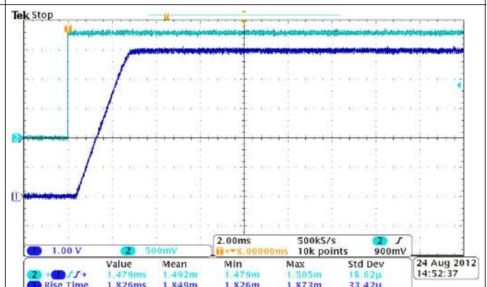
Figure 26. Turnon Response Time (V_{IN} = 5\text{ V}, V_{BIAS} = 5\text{ V}, C_{IN} = 1\text{ }\mu\text{F}, C_L = 0.1\text{ }\mu\text{F}, R_L = 10\text{ }\Omega) CH1: VOUT, CH2: ON
