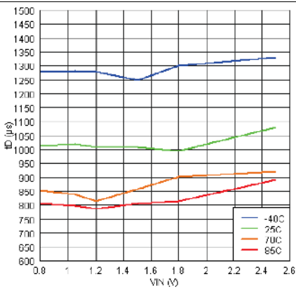
Figure 12. V_{IN} vs t_D ( V_{BIAS} = 2.5 V , C_T = 1 nF )
