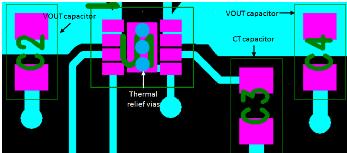
Figure 36. Layout Example
