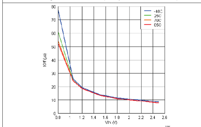
Figure 16. V_{IN} vs t_{OFF} ( V_{BIAS} = 2.5\text{ V} , C_T = 1\text{ nF} )
