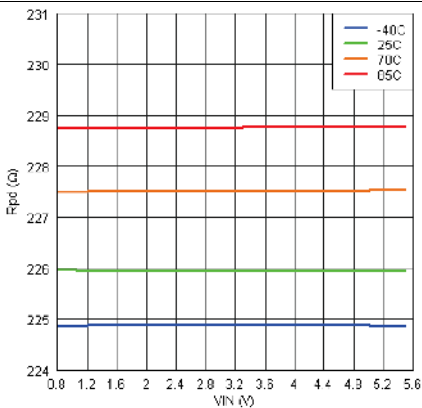
Figure 10. V_{IN} vs R_{PD} ( V_{BIAS} = 5.5 V )
