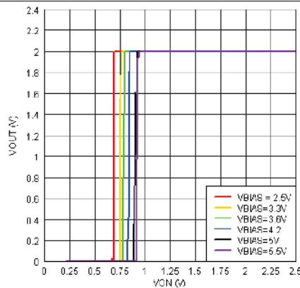
Figure 11. V_{ON} vs V_{OUT} ( T_A = 25^\circ C )
