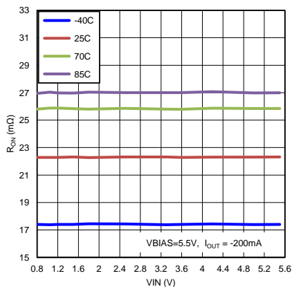
Figure 8. V_{IN} vs R_{ON} ( V_{BIAS} = 5.5 V )
