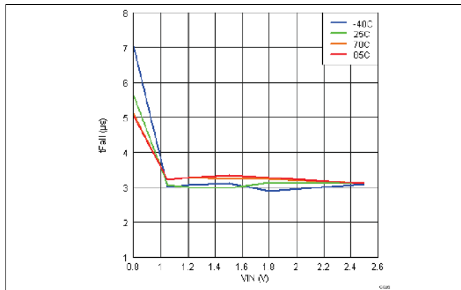
Figure 14. V_{IN} vs t_F ( V_{BIAS} = 2.5\text{ V} , C_T = 1\text{ nF} )
