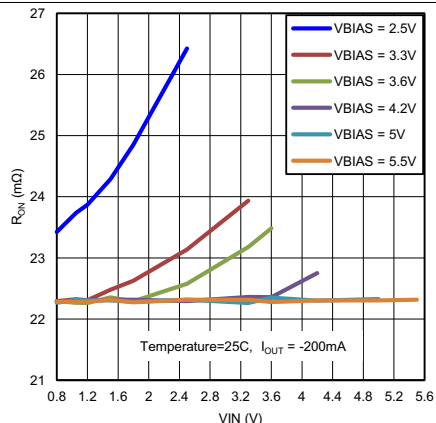
Figure 9. V_{IN} vs R_{ON} ( T_A = 25^\circ C )
