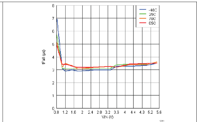
Figure 15. V_{IN} vs t_F ( V_{BIAS} = 5.5\text{ V} , C_T = 1\text{ nF} )
