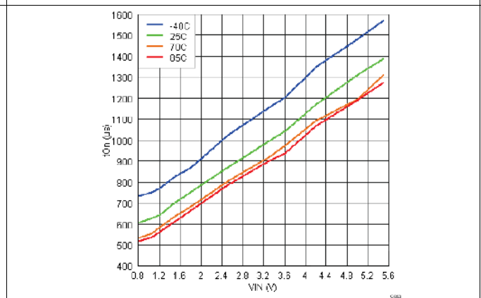
Figure 19. V_{IN} vs t_{ON} ( V_{BIAS} = 5.5\text{ V} , C_T = 1\text{ nF} )
