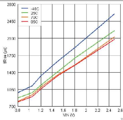
Figure 20. V_{IN} vs t_R ( V_{BIAS} = 2.5\text{ V} , C_T = 1\text{ nF} )
