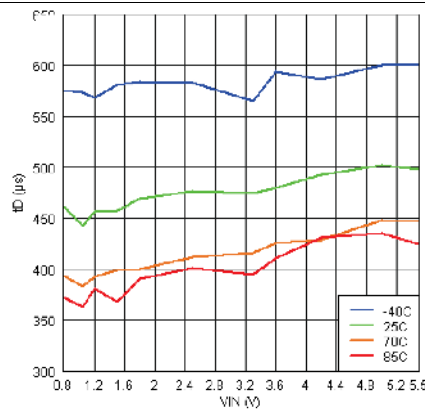
Figure 13. V_{IN} vs t_D ( V_{BIAS} = 5.5 V , C_T = 1 nF )
