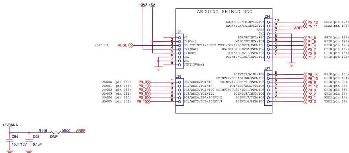
Figure 19: Arduino Shield interface
