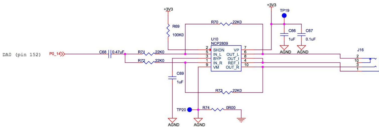
Figure 16: Audio output
