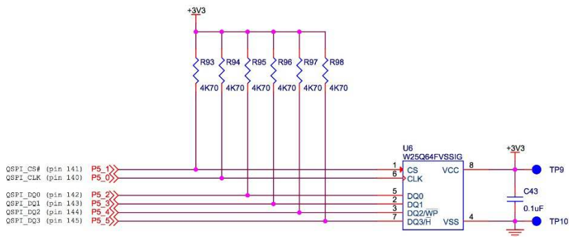
Figure 18: QSPI flash
