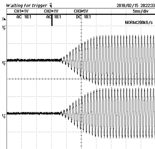
Figure 19. Advanced Switch 1
