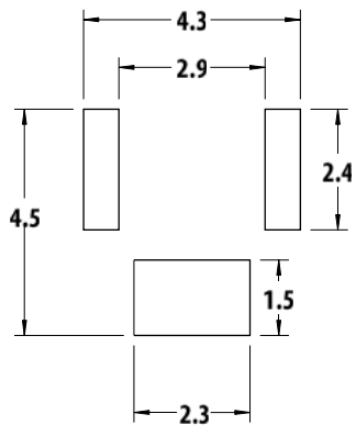
Figure 11: Recommended Soldering Land Pattern
