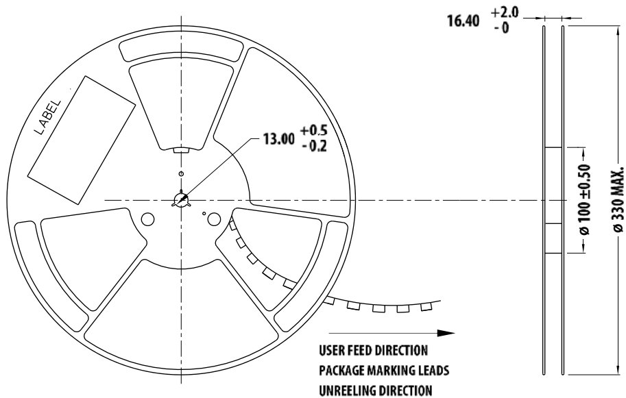
Figure 13: Reel Dimensions
