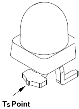
Figure 16: Solder Point Temperature on PCB
