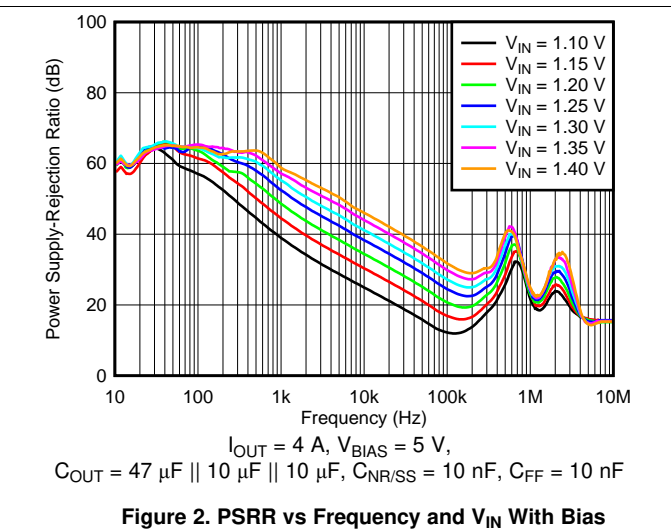
Figure 2. PSRR vs Frequency and V_{IN} With Bias
