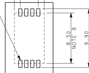
SMT PCB FOOTPRINT
