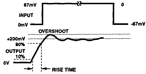
FIGURE 2. TRANSIENT RESPONSE
