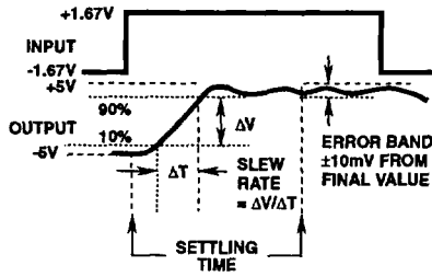
FIGURE 1. SLEW RATE AND SETTLE TIME
