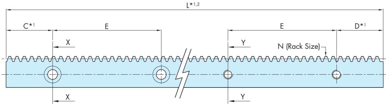
Rack with Counterbored Holes
