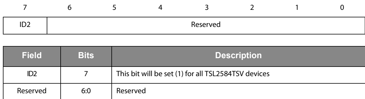
Figure 27: ID2 Register
