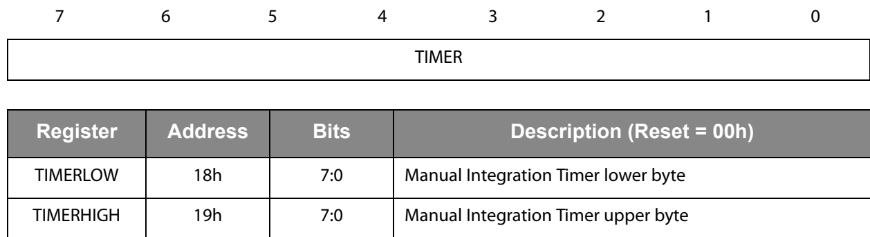
Figure 26: Manual Integration Timer Registers
