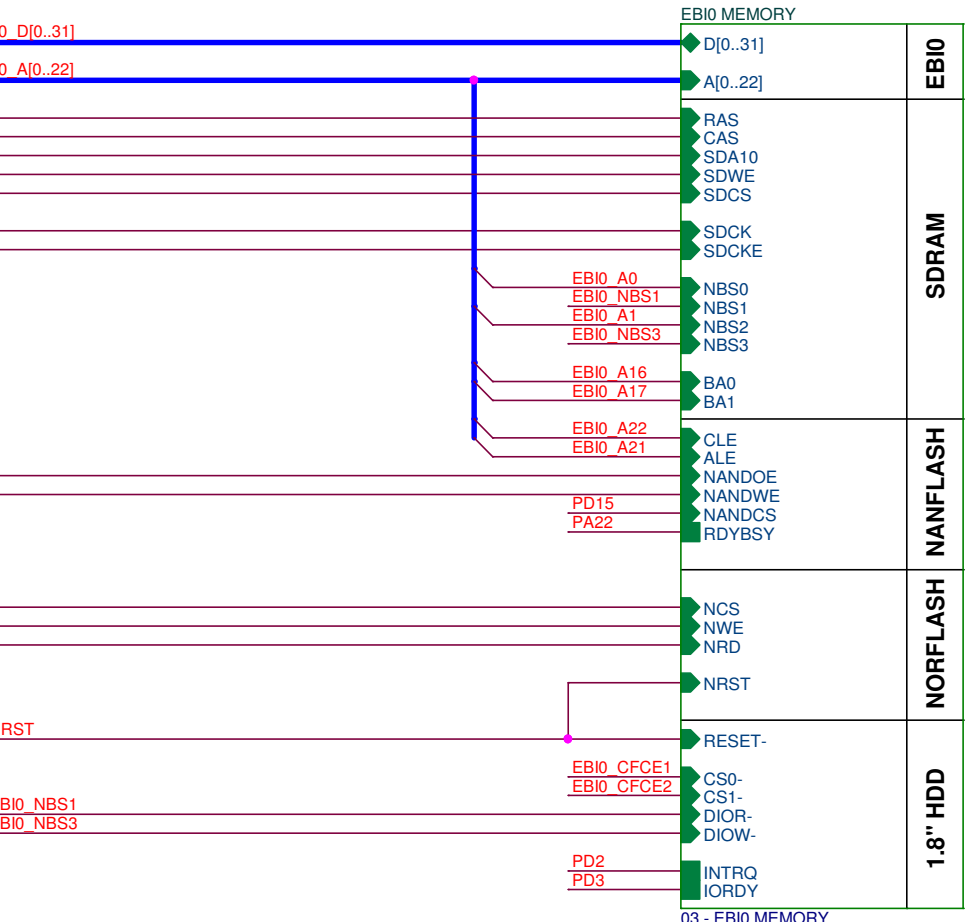
03 - EBIO MEMORY
