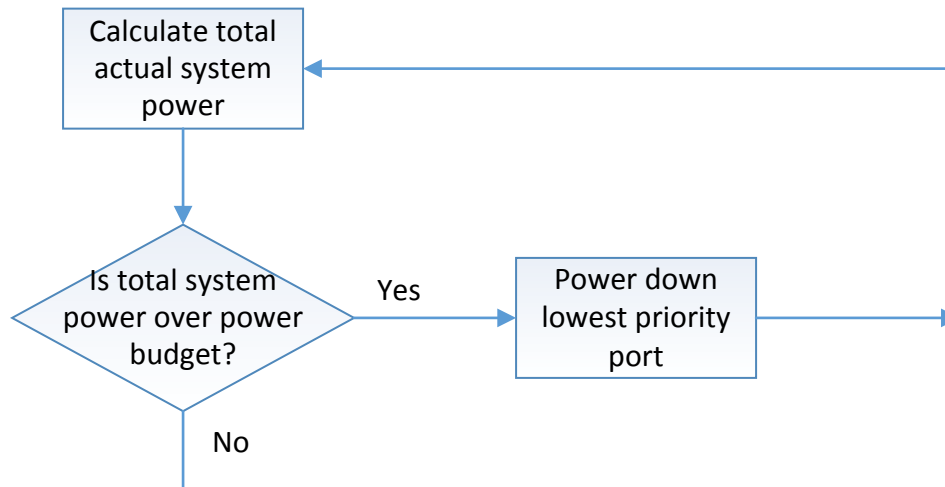
Figure 13. System Power Monitor Flow Chart
