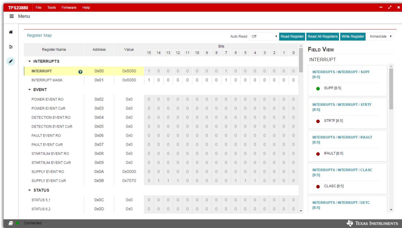
Figure 6. Register Map
