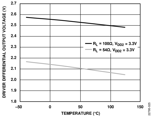
Figure 18. Driver Differential Output Voltage vs. Temperature
