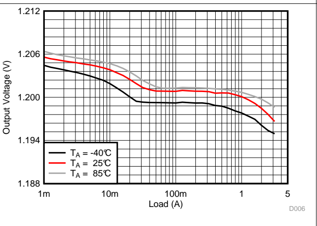
Figure 10. Load Regulation
