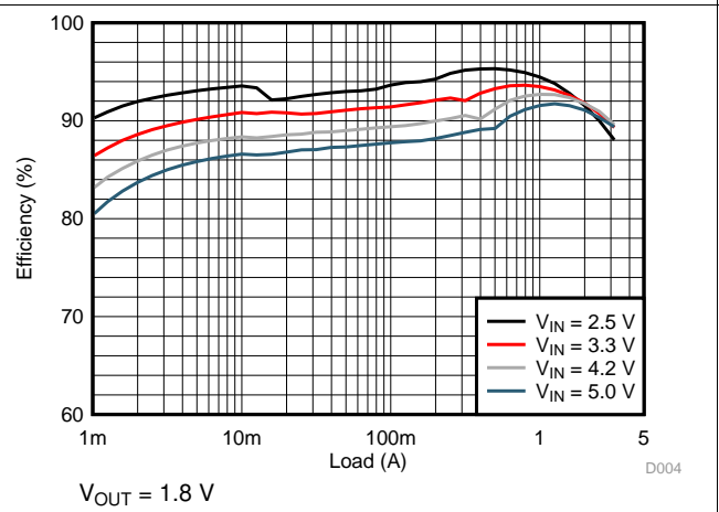
Figure 8. Efficiency
