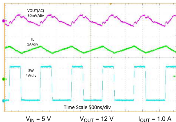
Figure 9-4. Switching Waveforms in CCM
