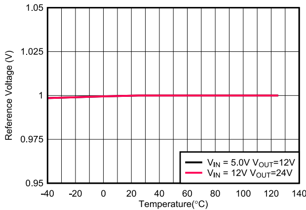
Figure 7-9. Reference Voltage vs Temperature
