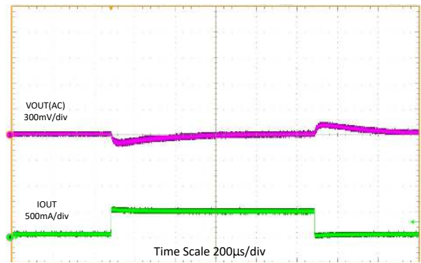
Figure 9-9. Load Transient ( I_{OUT} = 0.1 to 0.5 A)
