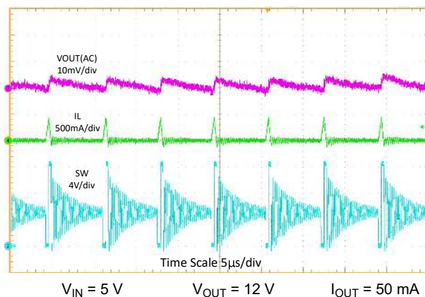
Figure 9-5. Switching Waveforms in 50-mA Load
