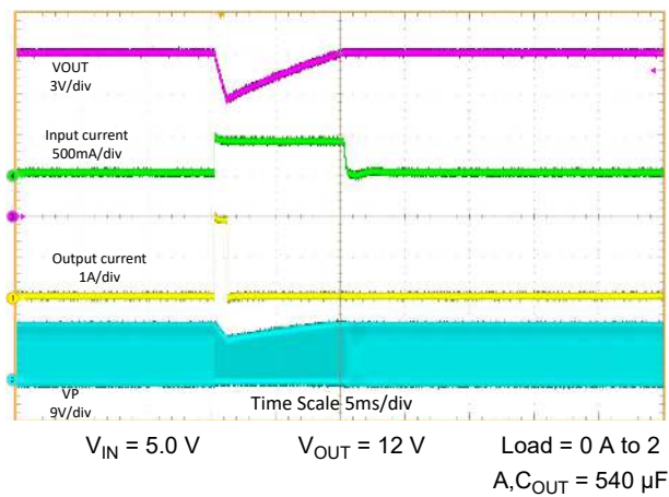
Figure 9-7. 2-A Load Pulse with ICL 500-mA
