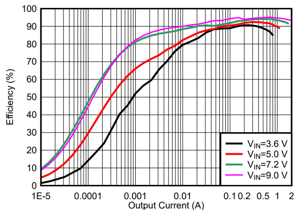
Figure 7-1. Efficiency vs Output Current V OUT = 12 V
