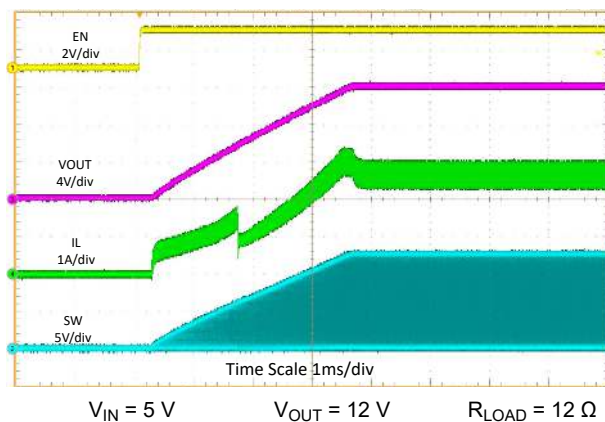
Figure 9-2. Start-Up Waveforms
