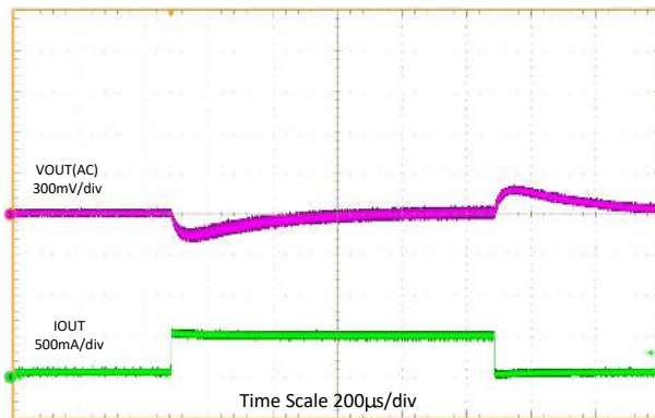
Figure 9-8. Load Transient ( I_{OUT} = 0.1 to 0.5 A)
