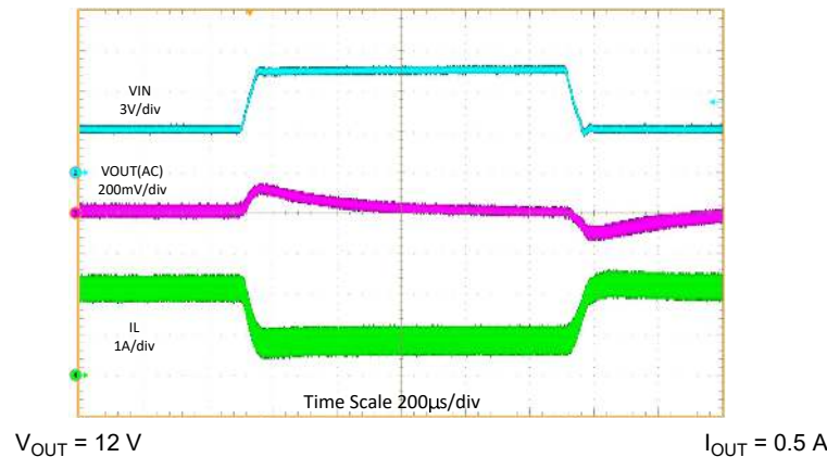
Figure 9-10. Line Transient ( V_{IN} = 3.3 V to 8.4 V)
