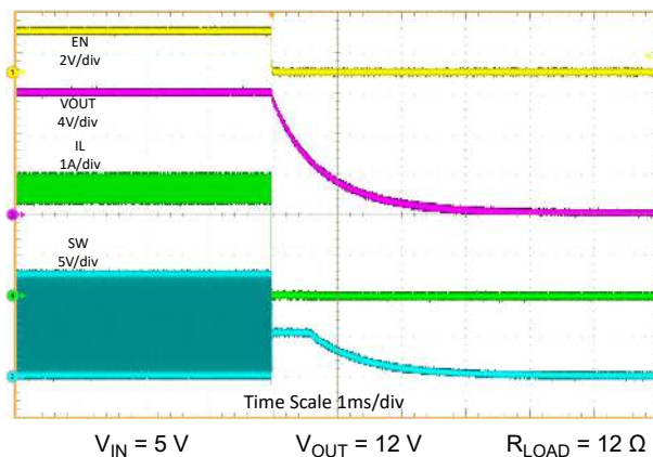
Figure 9-3. Shutdown Waveforms
