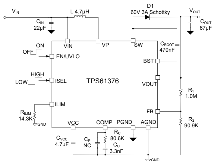
Figure 9-1. TPS61376 3.3-V to 8.4-V V_{IN} ; 12V V_{OUT} 0.5-A Output Converter
