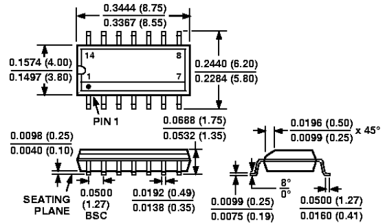
14-Pin SOIC (SO-14)
