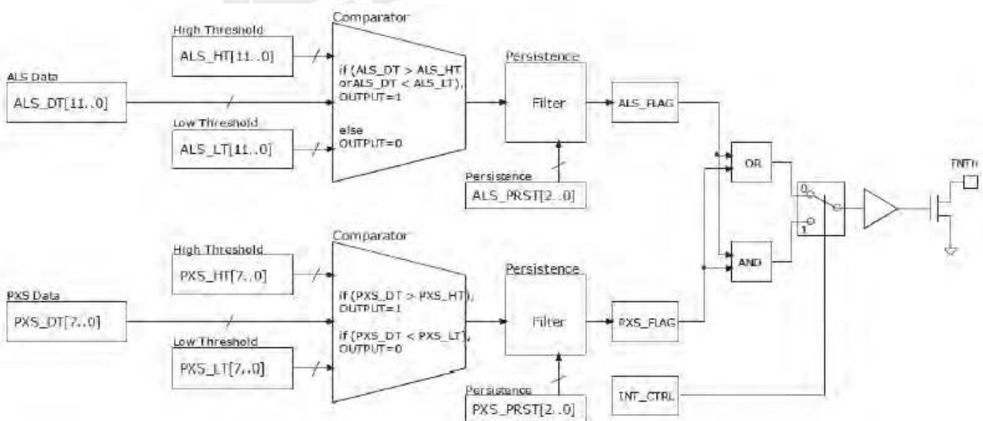
Figure 6. Interrupt operation
