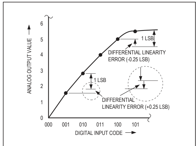
Figure 14b. Differential Nonlinearity
