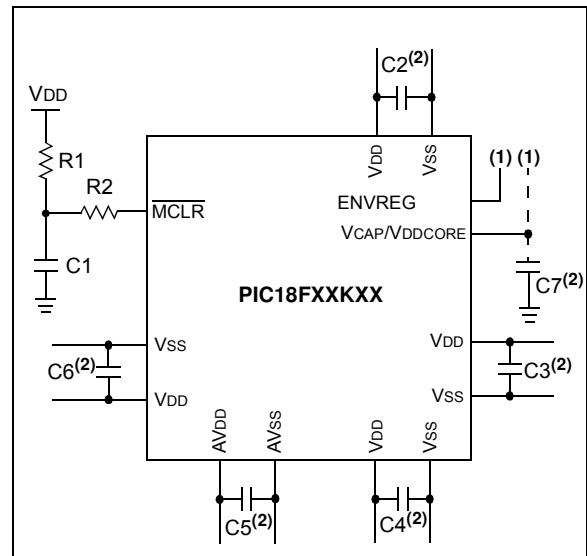
FIGURE 2-1: RECOMMENDED MINIMUM CONNECTIONS
