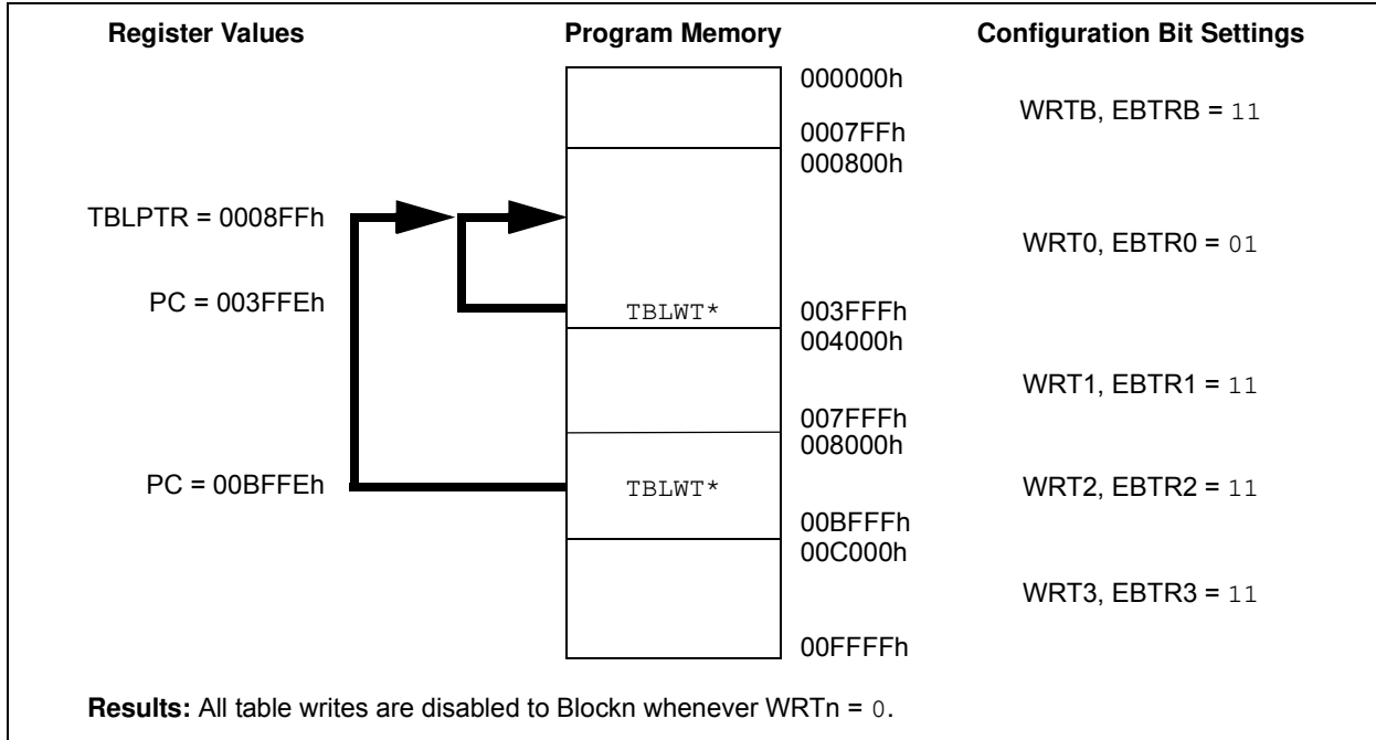
FIGURE 28-7: TABLE WRITE (WRTn) DISALLOWED
