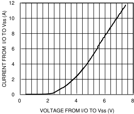
Figure 5 Current vs. Voltage
