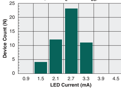
Typical I_C for Switch Dropout (N=50, I_L=250mA_{DC} )
