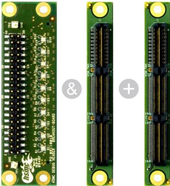
Debug HSMC Card
