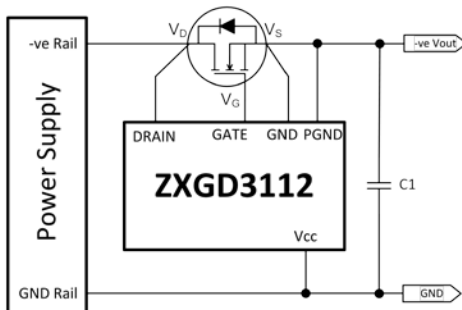
Typical Configuration for Low-Side -ve Supply Rail
