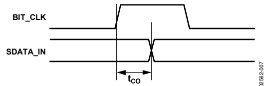
Figure 7. Propagation Delay
