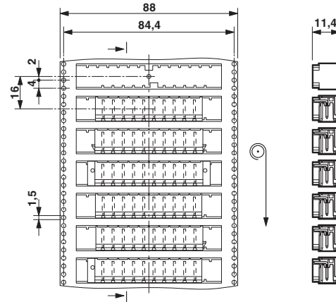
Dimensioned drawing
