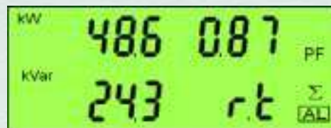
Example of variables displayed with serial communication diagnostics: r.t (Rx/Tx)
