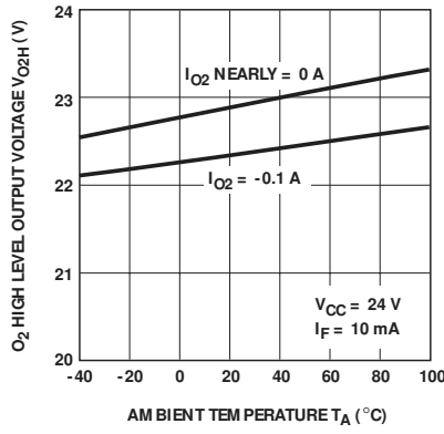
Figure 27. Typical high level output 2 voltage vs. ambient temperature, HCPL-3100.
