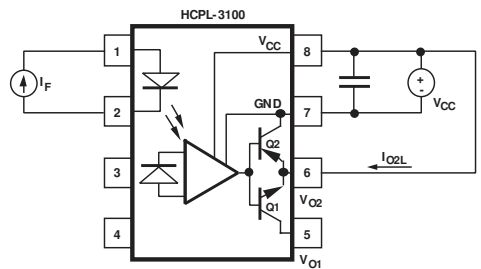
Figure 6. Test circuit for leakage current I_{O2L} .
