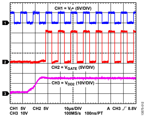
Figure 12. Typical V_{DD2} Startup to Output Valid
