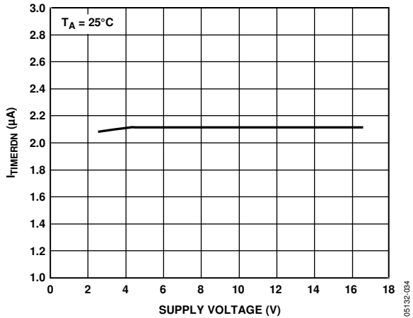
Figure 18. I_{TIMERDN} (in Cool-Off Cycle) vs. Supply Voltage
