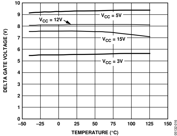
Figure 13. Delta GATE Voltage vs. Temperature
