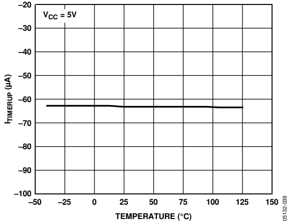
Figure 17. I_{TIMERUP} (During Cct Breaker Delay) vs. Temperature
