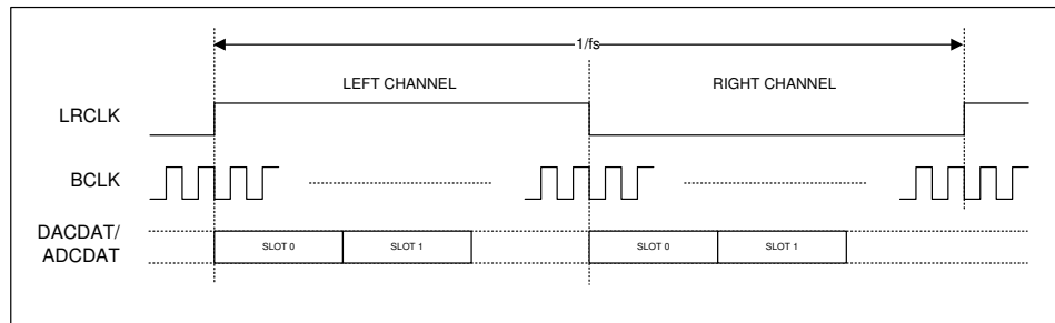
Figure 51 TDM in Left-Justified Mode
