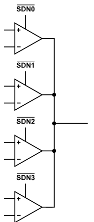
Figure 54. Four AD8231s in Multiplexing Configuration
