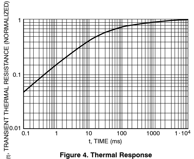
Figure 4. Thermal Response
