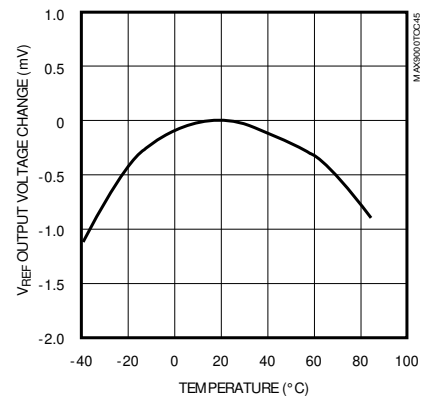
V_{REF} OUTPUT VOLTAGE CHANGE vs. TEMPERATURE
