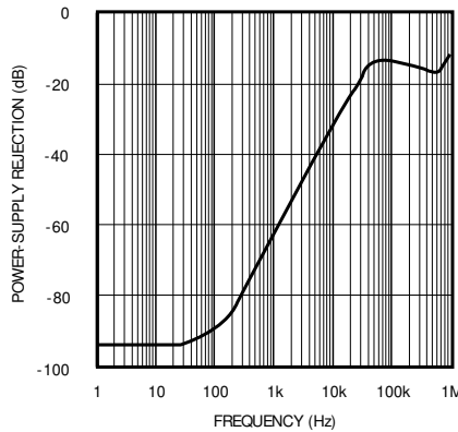
V_{REF} POWER-SUPPLY REJECTION vs. FREQUENCY
