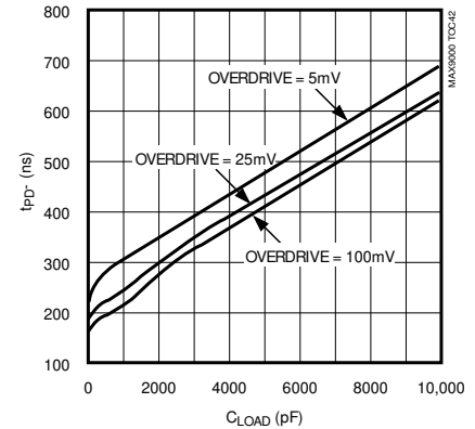
NEGATIVE COMPARATOR PROPAGATION DELAY ( t_{PD-} ) vs. LOAD CAPACITANCE
