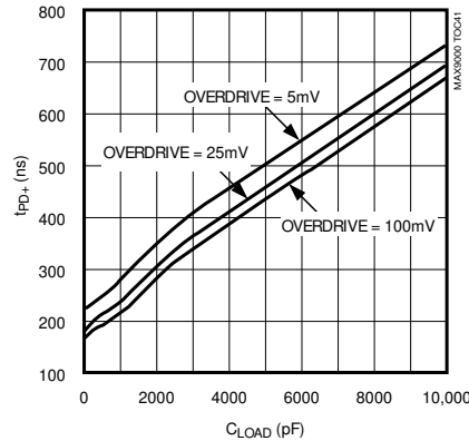
POSITIVE COMPARATOR PROPAGATION DELAY ( t_{PD+} ) vs. LOAD CAPACITANCE
