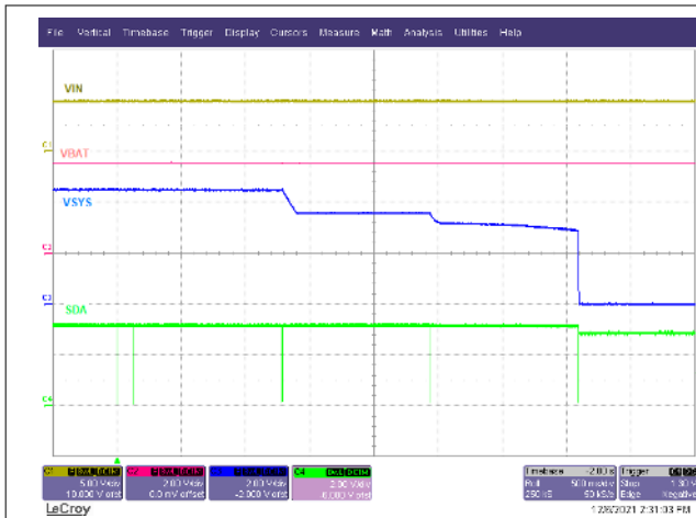
SYS_MODE = 00 → 01 → 10 → 11
