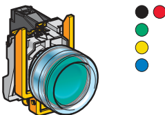
Booted flush push XB4BP●1/BP42 see page 27
