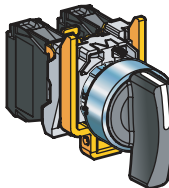
Long handle, black XB4BJ●● see page 39
