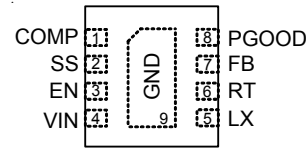
WDFN-8L 3x3
