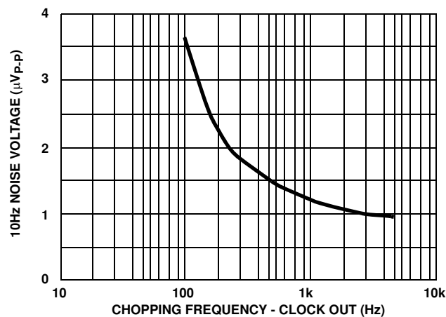
FIGURE 12. 10Hz NOISE VOLTAGE vs CHOPPING FREQUENCY
