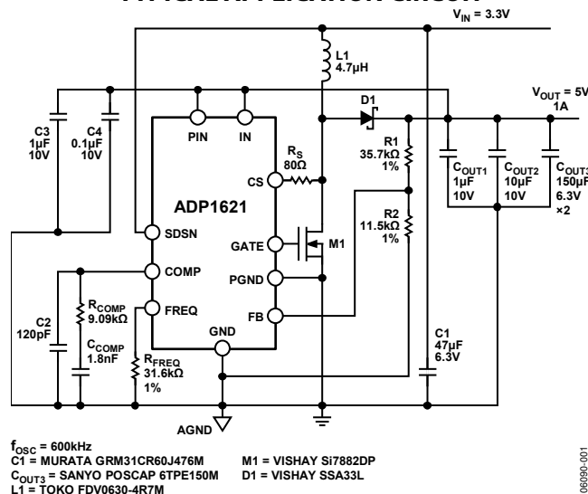
Figure 1. High Efficiency Output Boost Converter in Lossless Mode, 3.3 V Input, 5 V Output (Bootstrapped)
