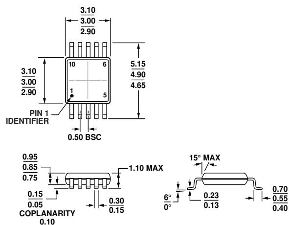
Figure 43. 10-Lead Mini Small Outline Package [MSOP]
