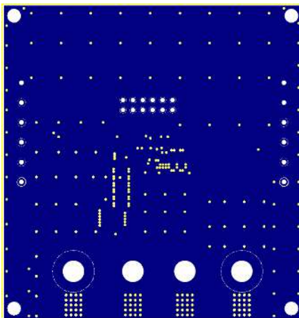
Figure 3: Inner Layer 1
