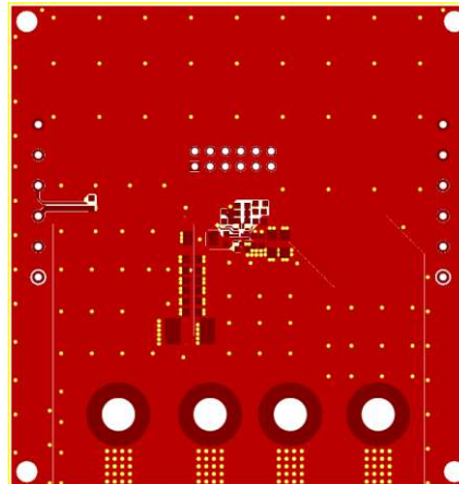
Figure 2: Top Layer
