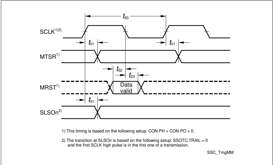
Figure 20 SSC Master Mode Timing
