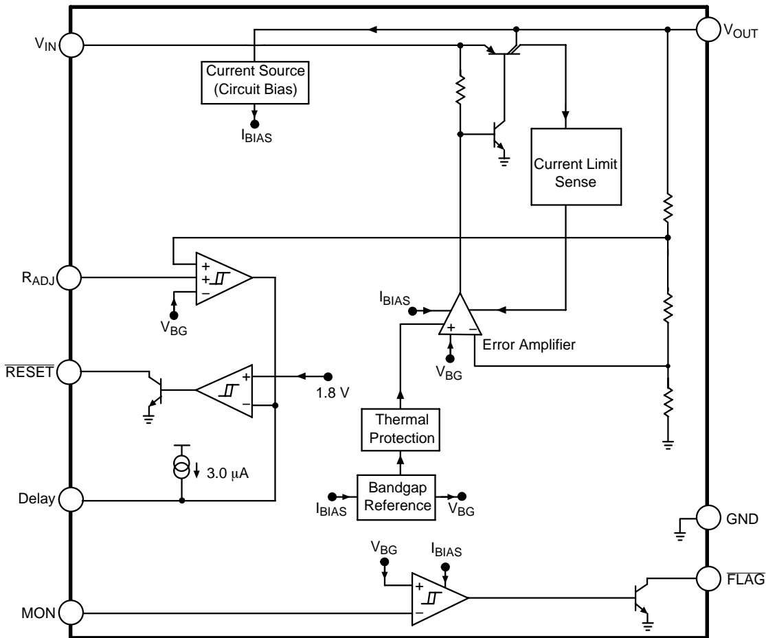
Figure 10. Block Diagram
