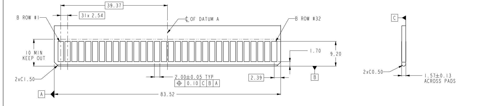
RECOMMENDED DAUGHTER CARD LAYOUT (TOP SIDE)
