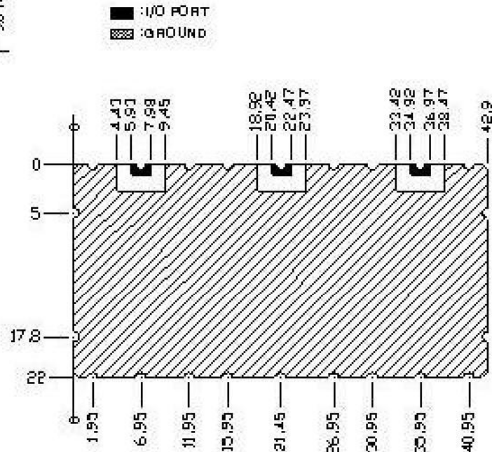
<BOTTOM VIEW>
