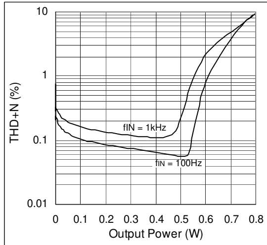
Figure 11. THD + Noise vs. Output Power; V_{DD} = 3V, R_L = 4\Omega, A_v = 4 V_{DD} = 3V, R_L = 8\Omega, A_v = 4
