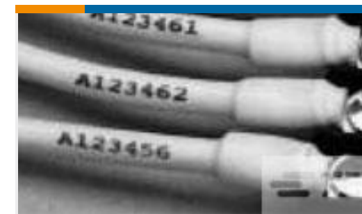
TE Part #5053324010 RNF-100-1-6-SP
